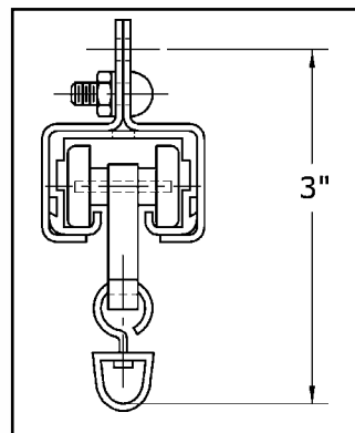
Cross Section of 113 Track Suspended Installation
