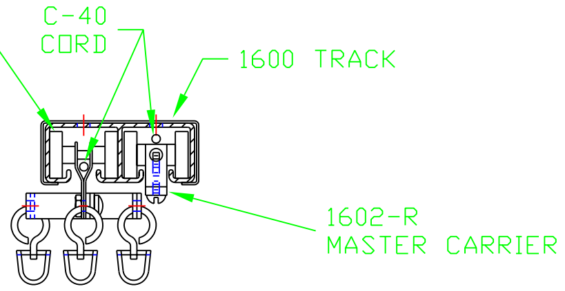
SECTION VIEW OF MASTER CARRIER
